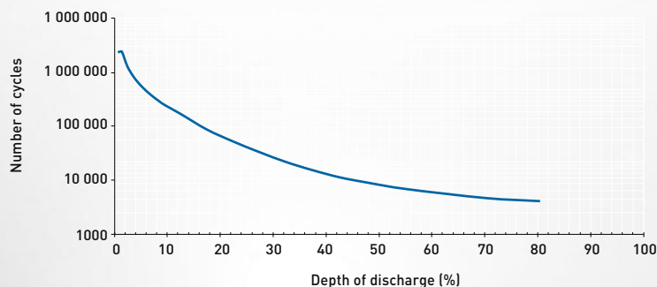
Typical lithium-ion cycling life after charge at 56 V
